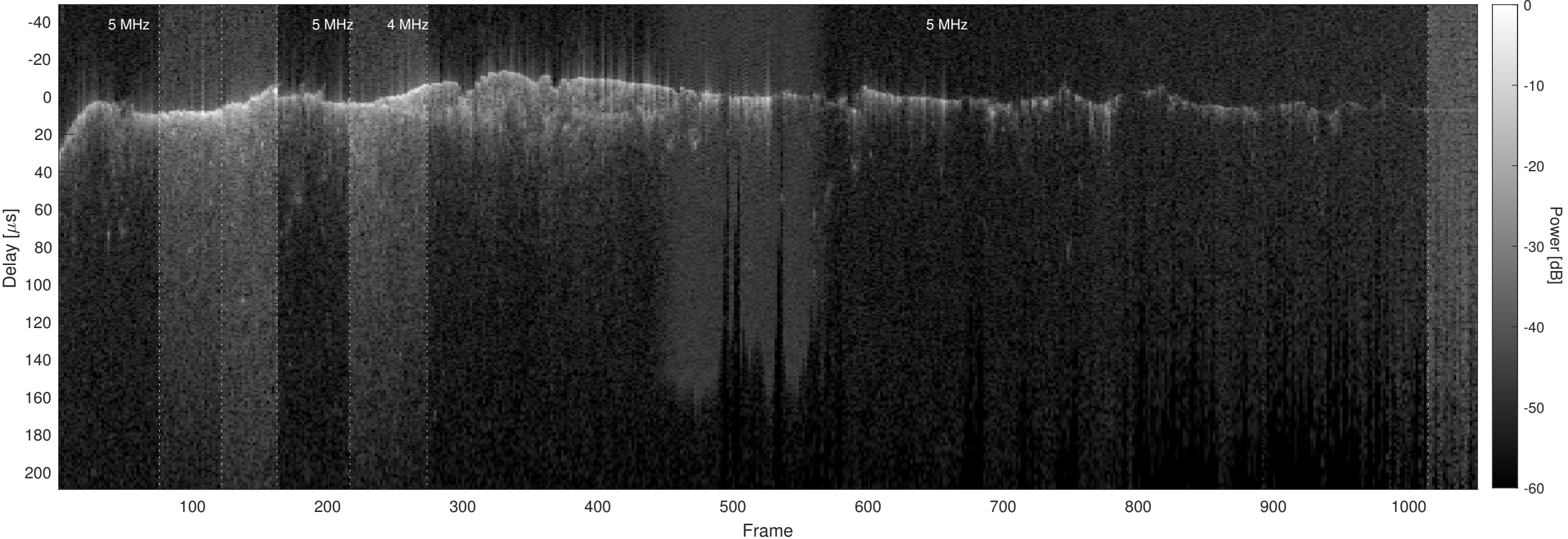
Orbit 2483, Optimized, No Window, Channel 2
