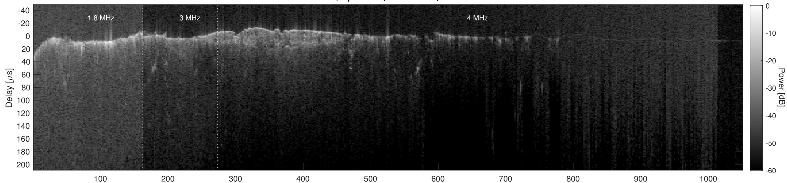
Orbit 2483, Cluttergram
