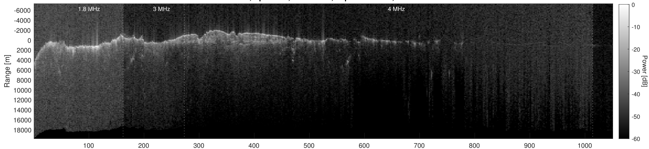
Orbit 2483, Depth-Corrected Cluttergram
