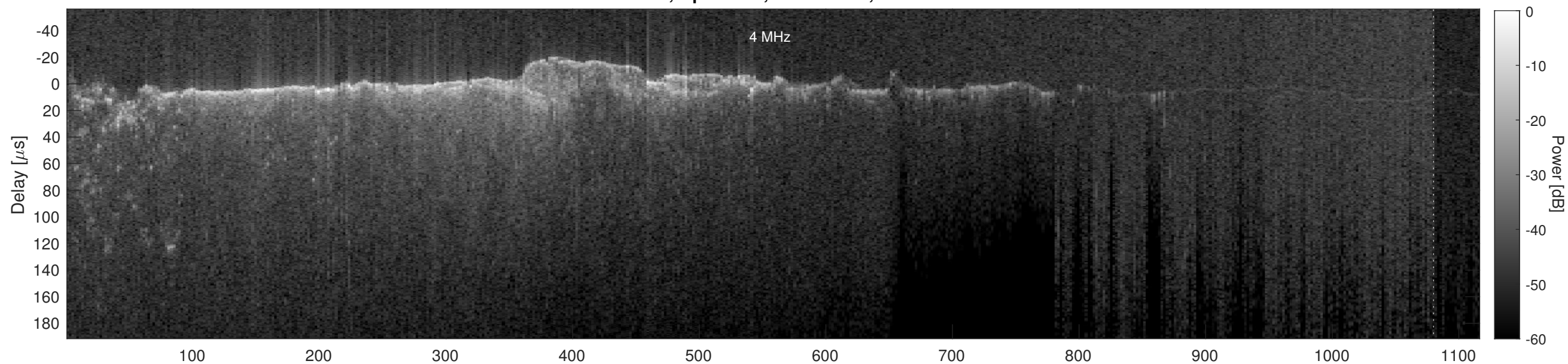
Orbit 2484, Cluttergram
