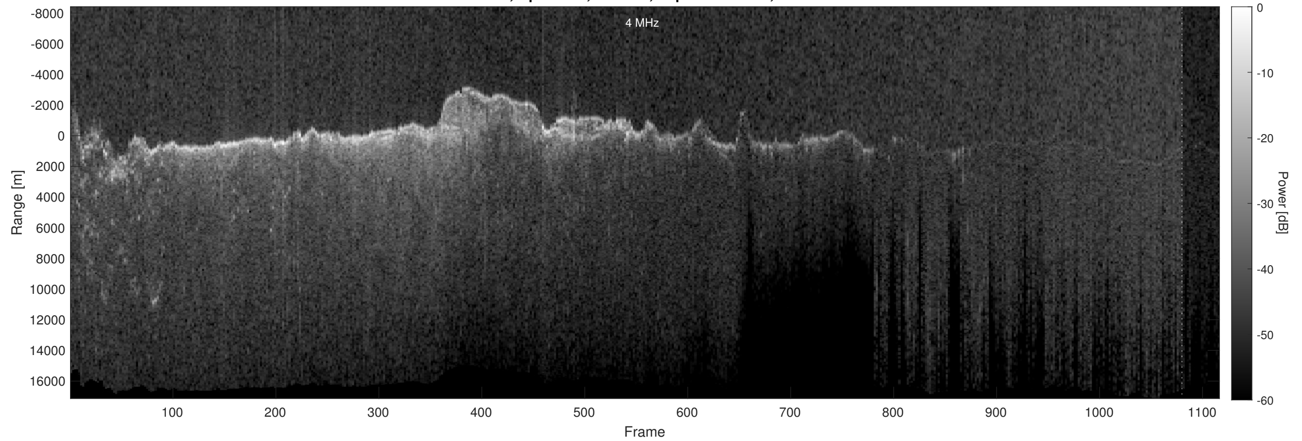
Orbit 2484, Optimized, Window, Depth-Corrected, Channel 2
