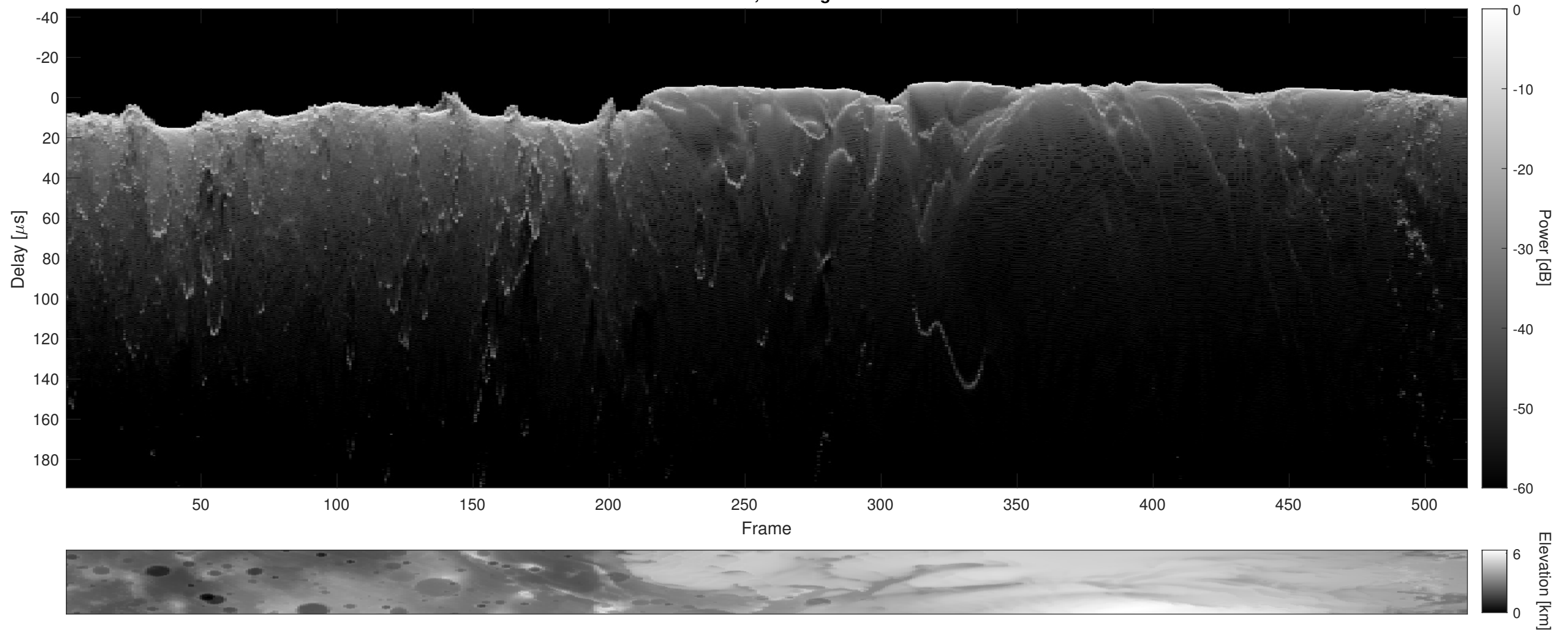
Orbit 2486, Cluttergram
