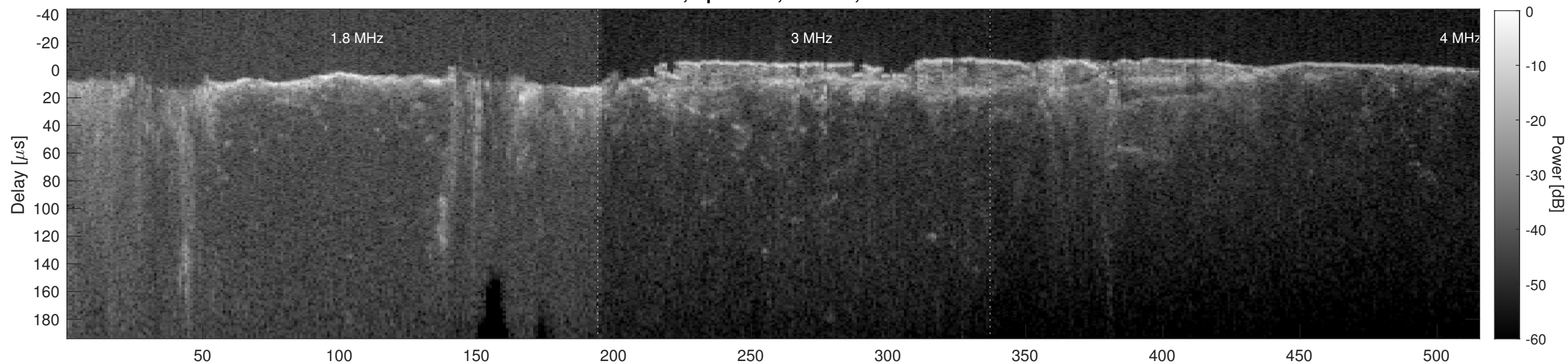
Orbit 2486, Cluttergram
