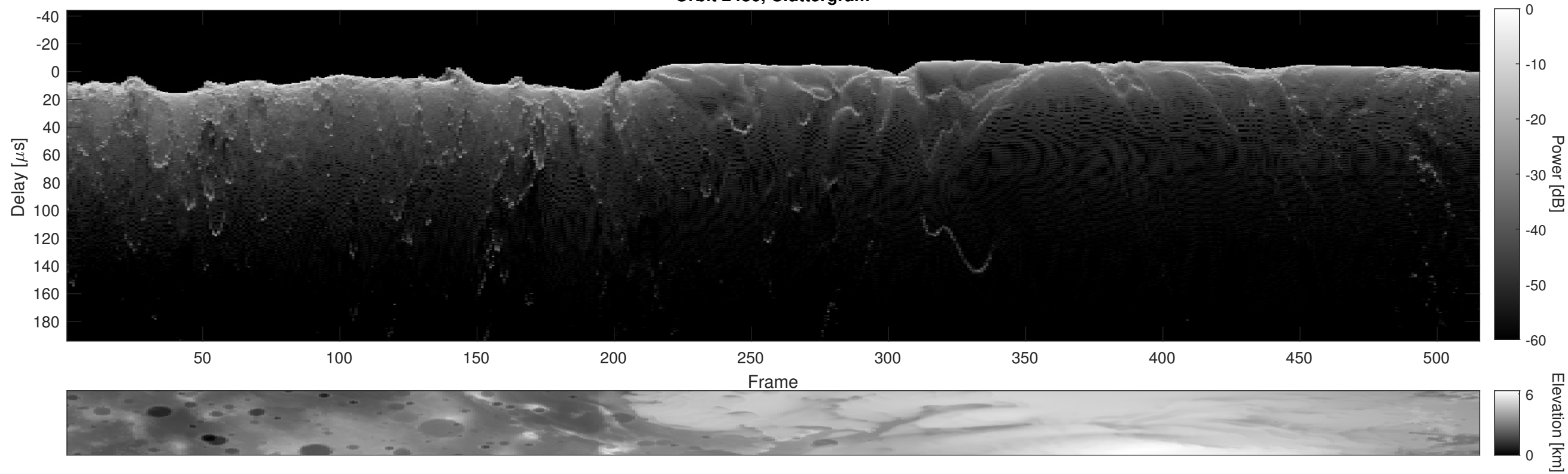
Orbit 2486, Cluttergram
