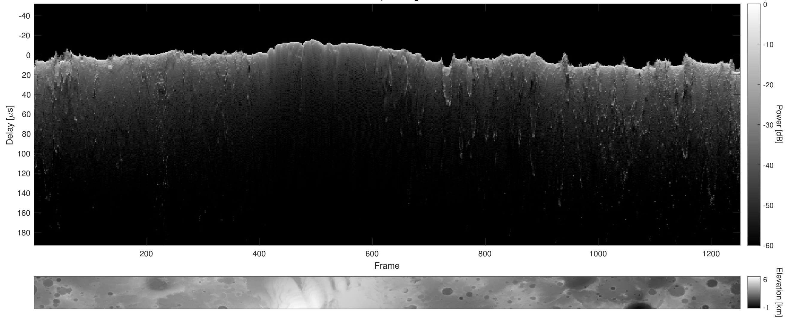
Orbit 2487, Cluttergram
