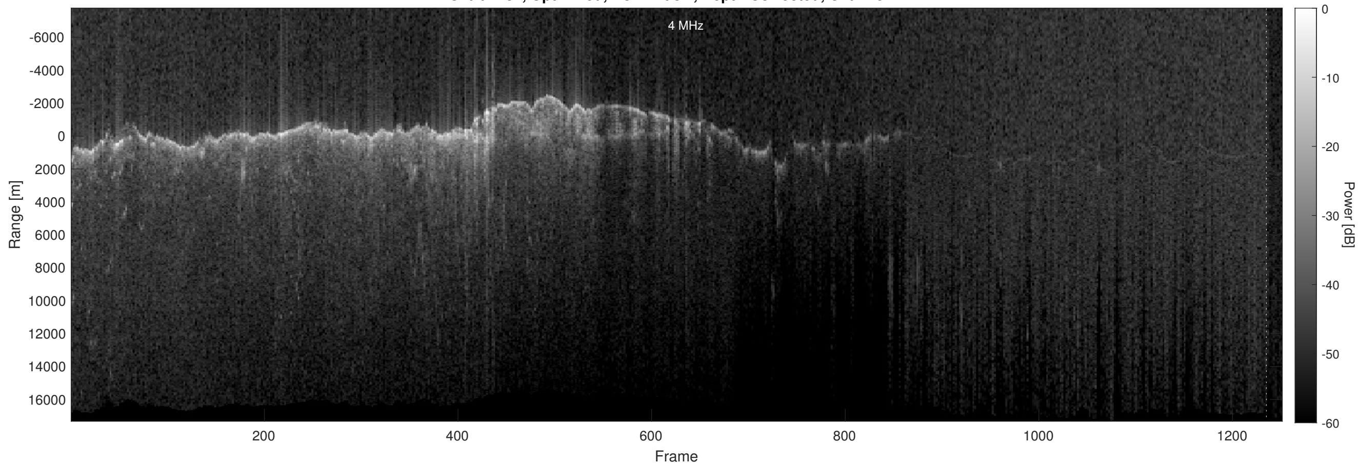
Orbit 2487, Optimized, No Window, Depth-Corrected, Channel 2
