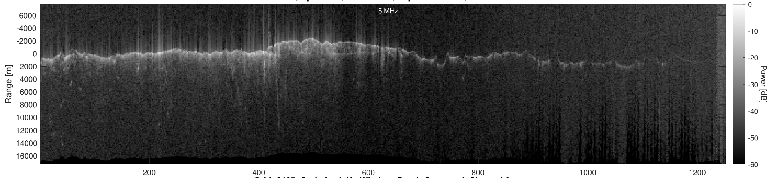
Orbit 2487, Optimized, No Window, Depth-Corrected, Channel 2
