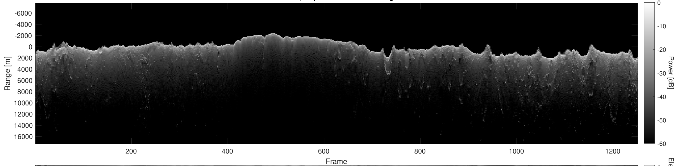
Orbit 2487, Depth-Corrected Cluttergram
