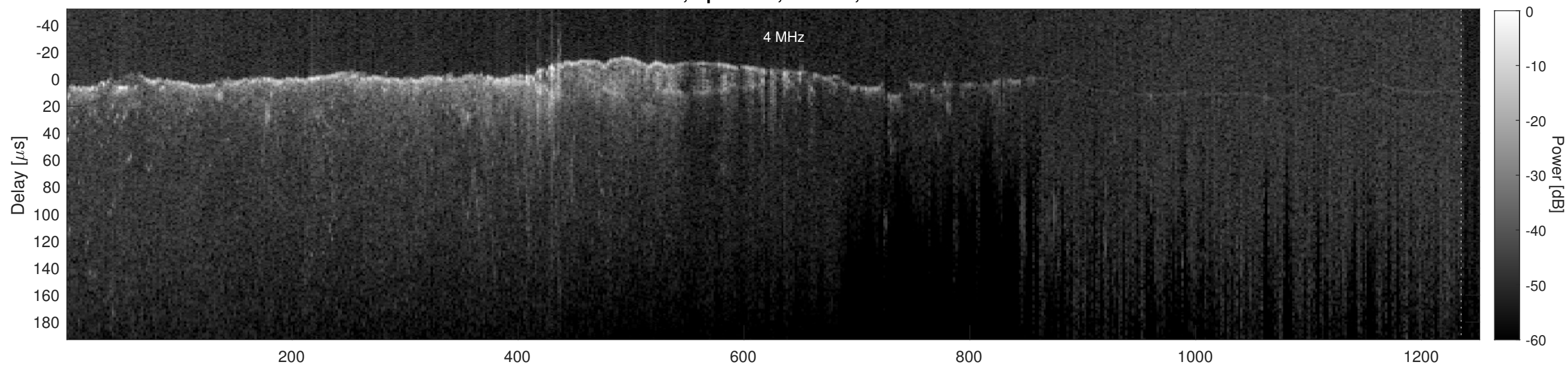
Orbit 2487, Cluttergram
