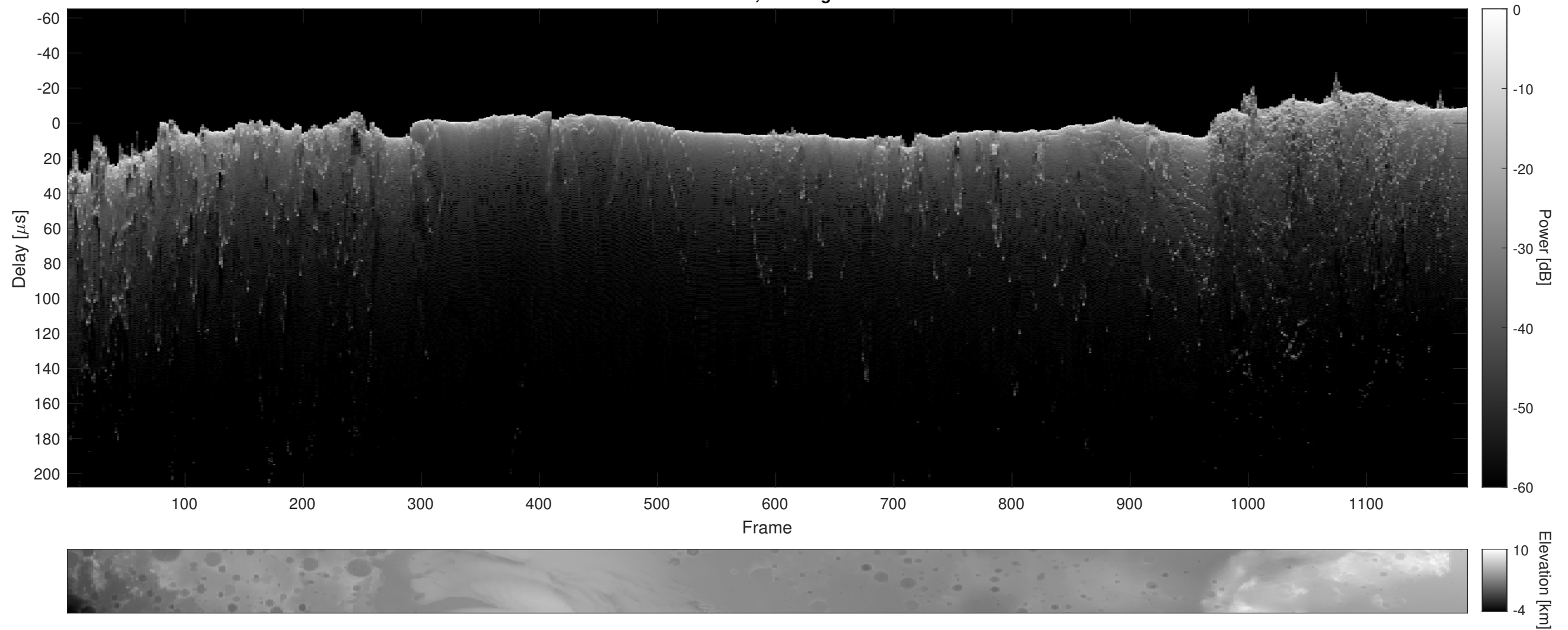
Orbit 2490, Cluttergram
