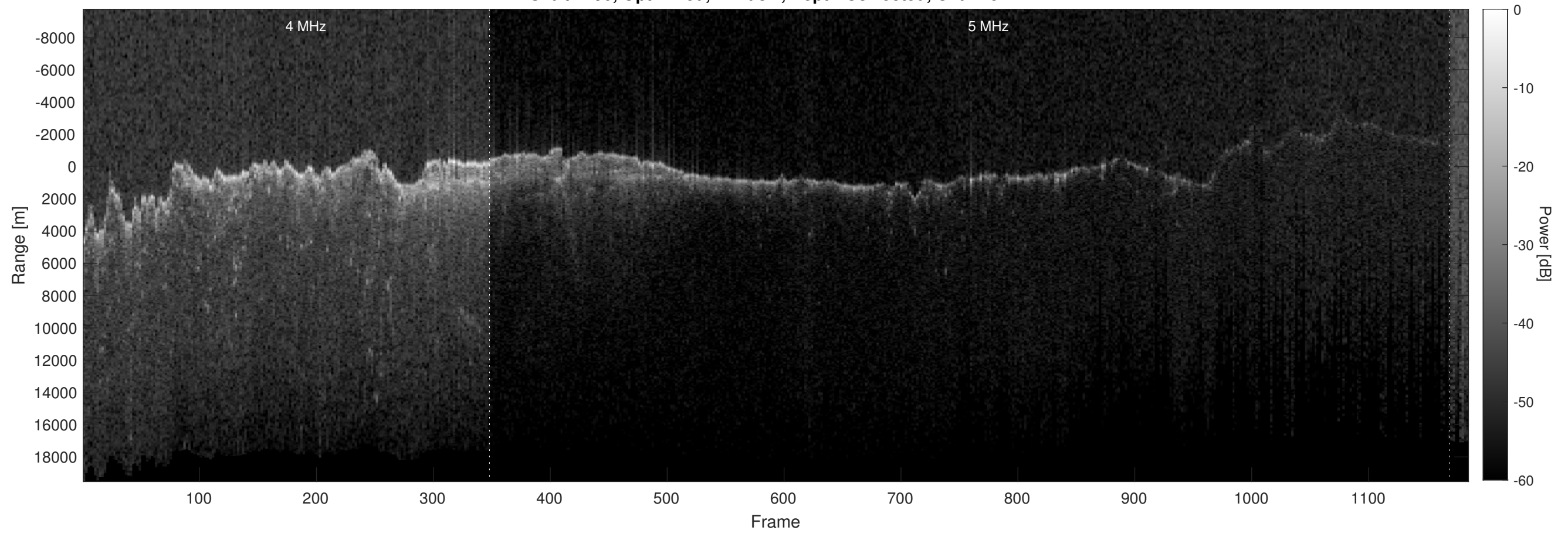
Orbit 2490, Optimized, Window, Depth-Corrected, Channel 2
