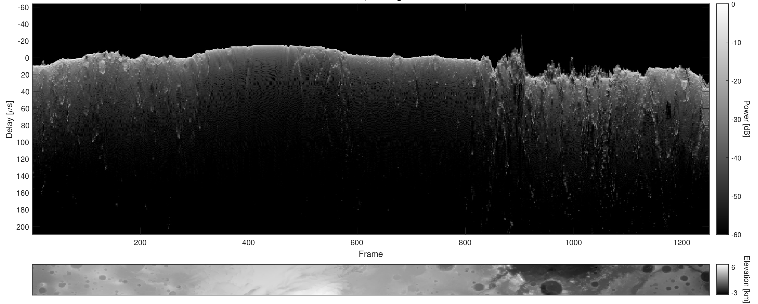
Orbit 2493, Cluttergram
