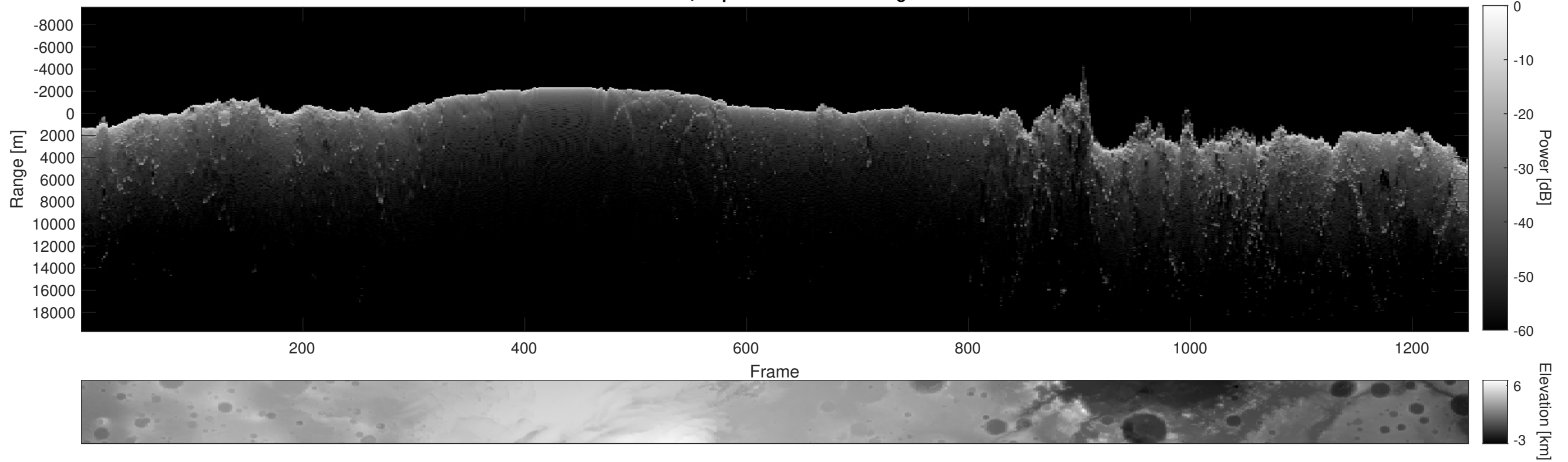
Orbit 2493, Depth-Corrected Cluttergram
