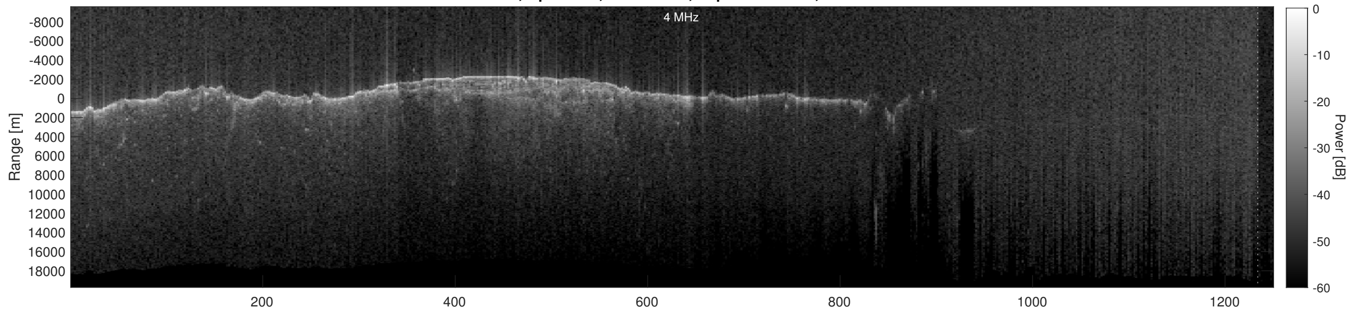
Orbit 2493, Depth-Corrected Cluttergram
