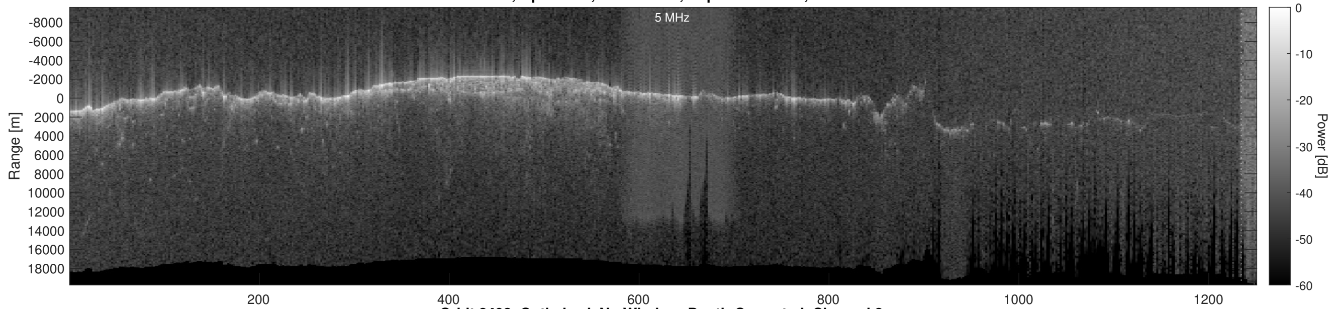
Orbit 2493, Optimized, No Window, Depth-Corrected, Channel 2
