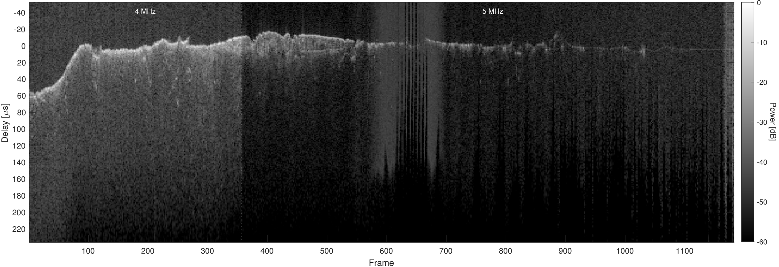
Orbit 2494, Optimized, Window, Channel 2
