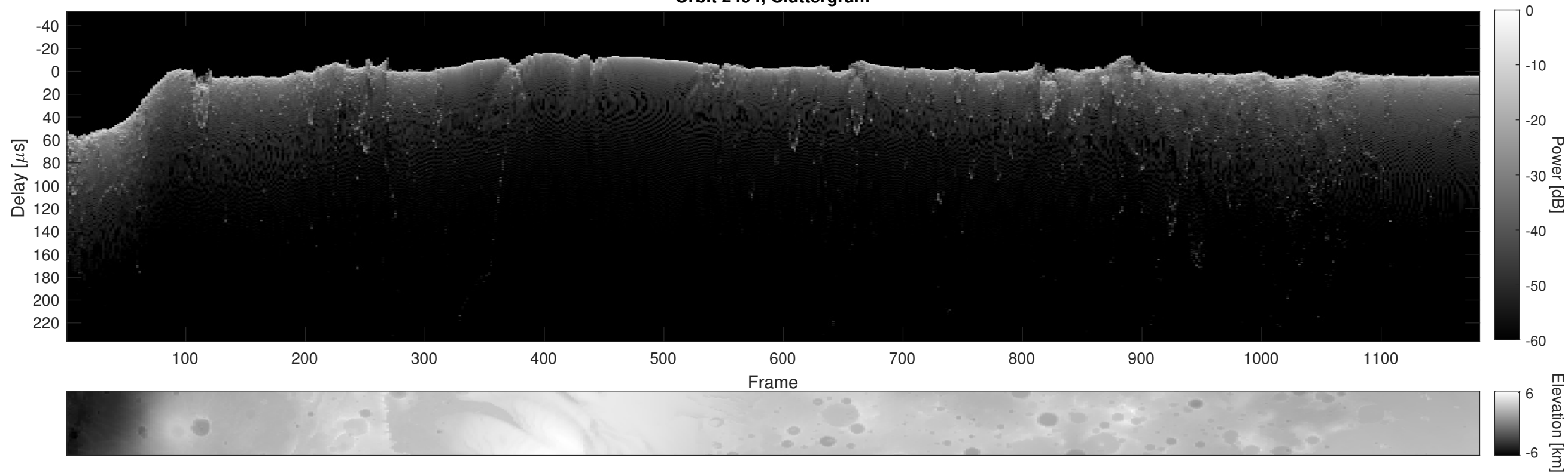
Orbit 2494, Cluttergram
