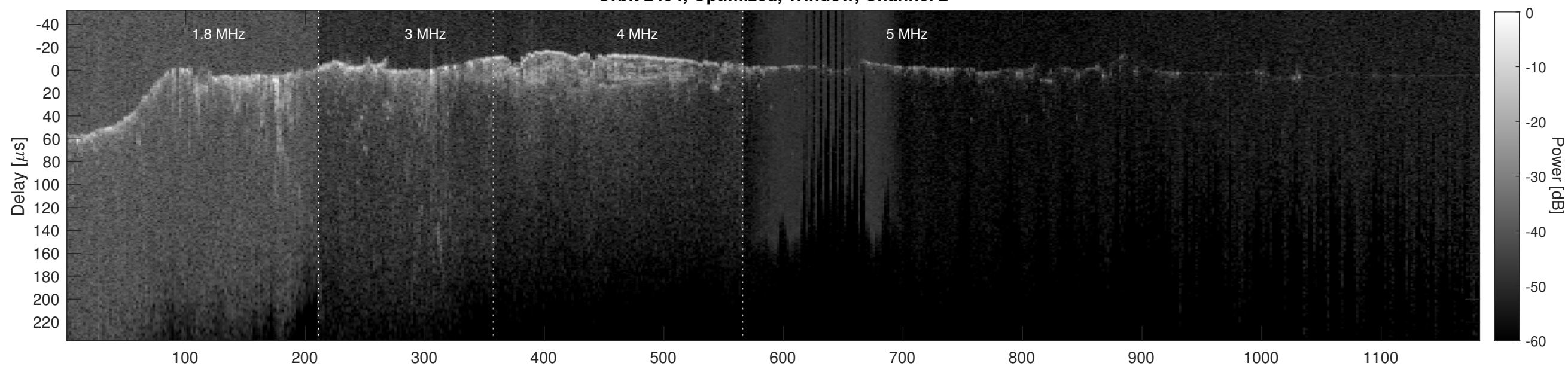
Orbit 2494, Cluttergram
