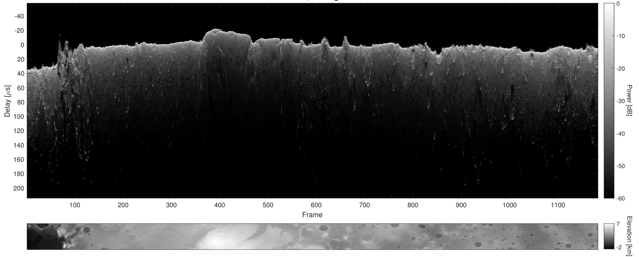
Orbit 2495, Cluttergram
