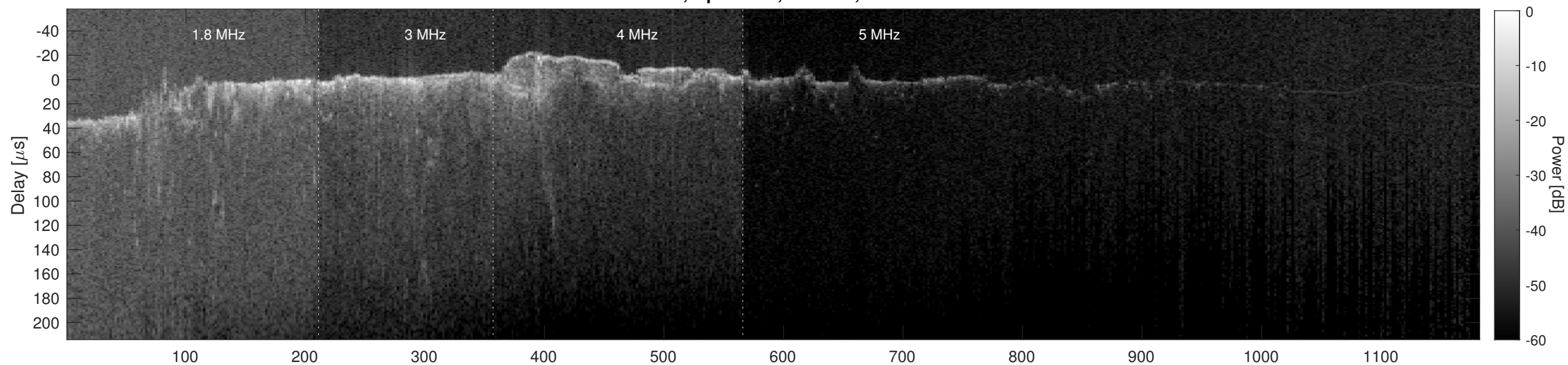
Orbit 2495, Cluttergram
