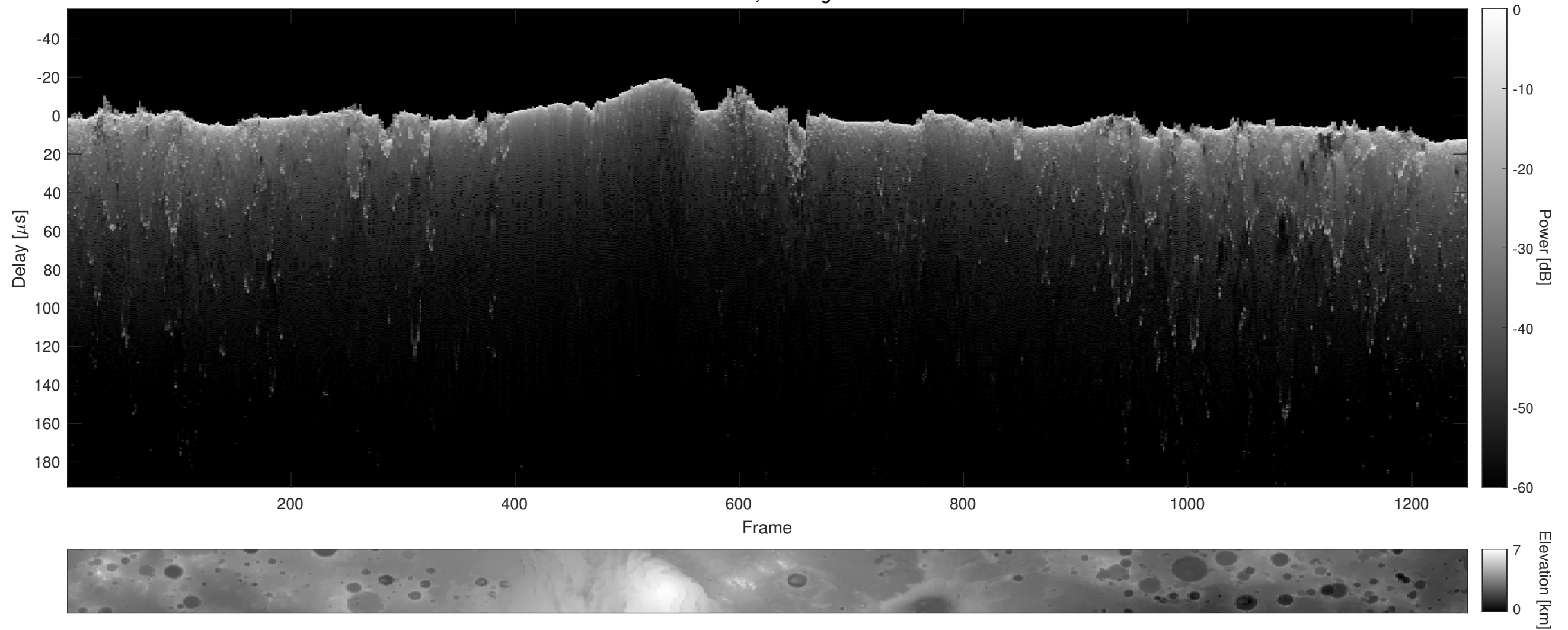
Orbit 2496, Cluttergram
