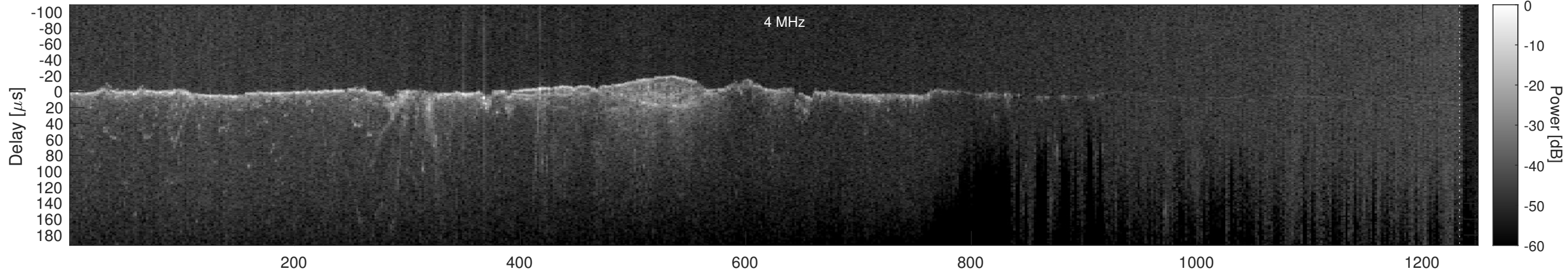
Orbit 2496, Cluttergram
