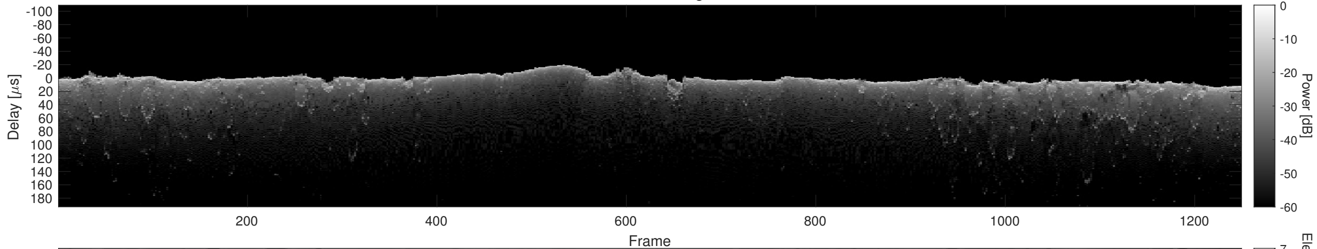
Orbit 2496, Cluttergram
