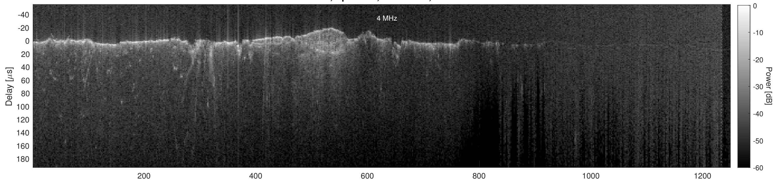
Orbit 2496, Cluttergram
