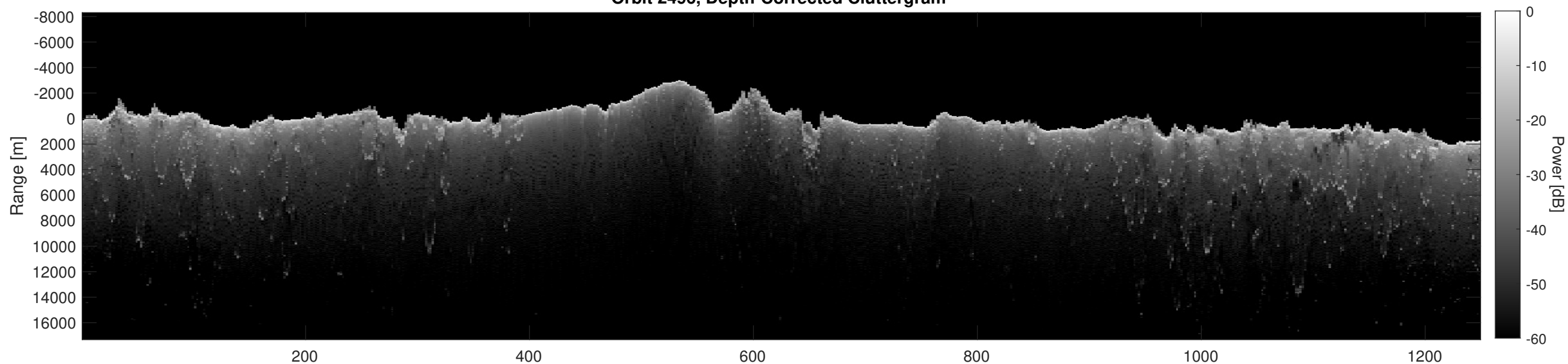
Orbit 2496, Depth-Corrected Cluttergram
