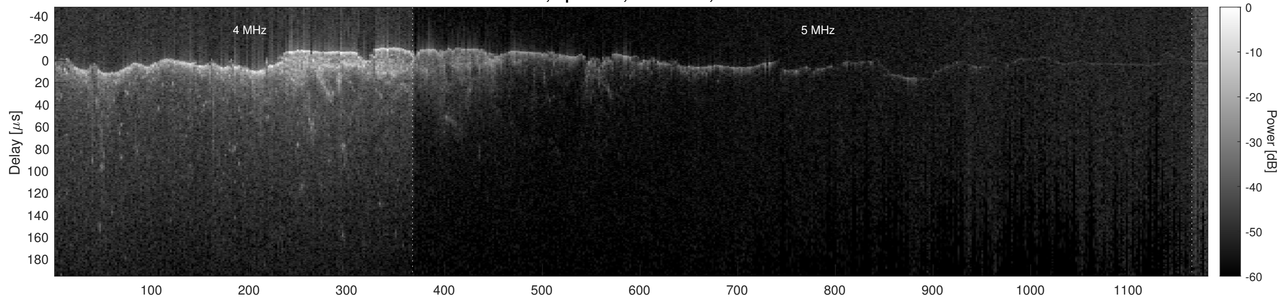
Orbit 2497, Optimized, No Window, Channel 2
