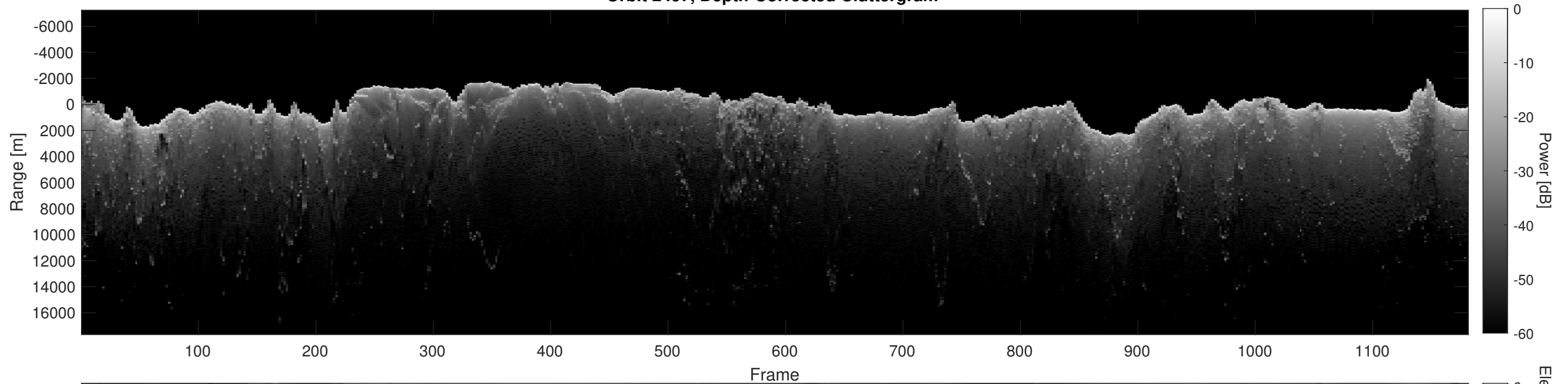
Orbit 2497, Depth-Corrected Cluttergram
