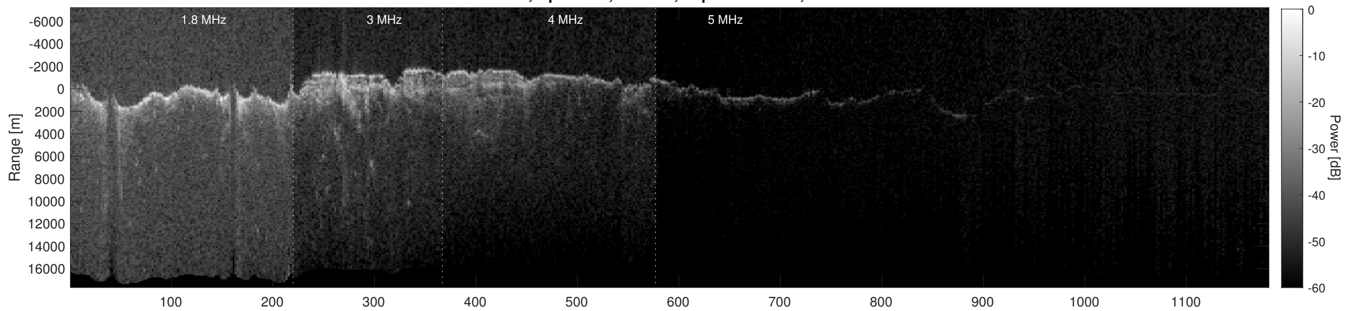
Orbit 2497, Depth-Corrected Cluttergram
