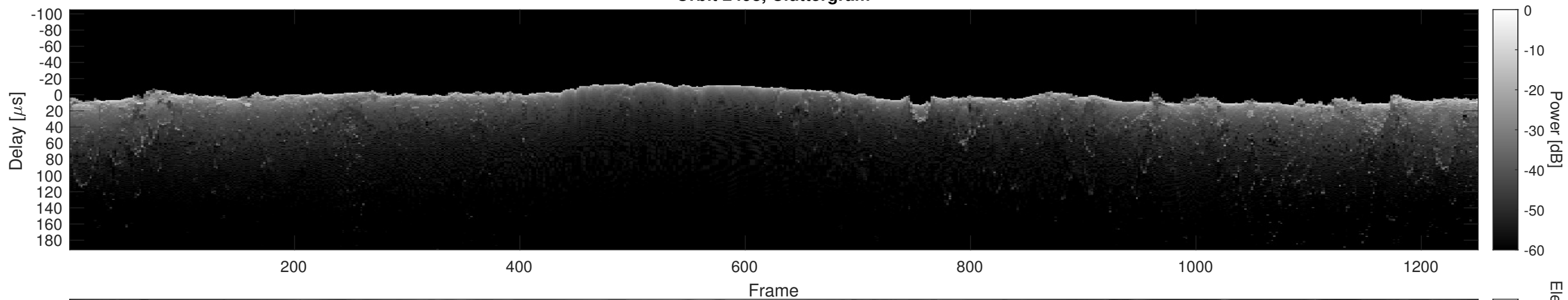
Orbit 2498, Cluttergram
