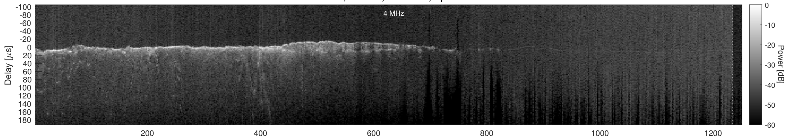
Orbit 2498, Cluttergram
