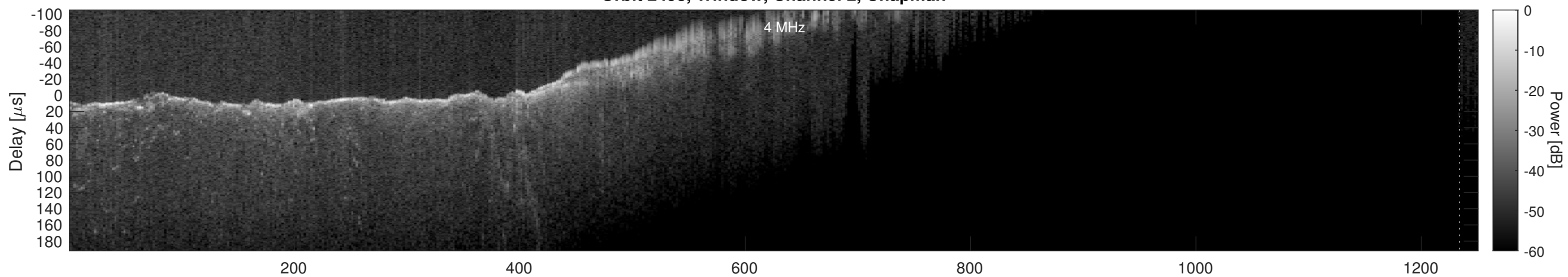
Orbit 2498, Window, Channel 2, Optimized
