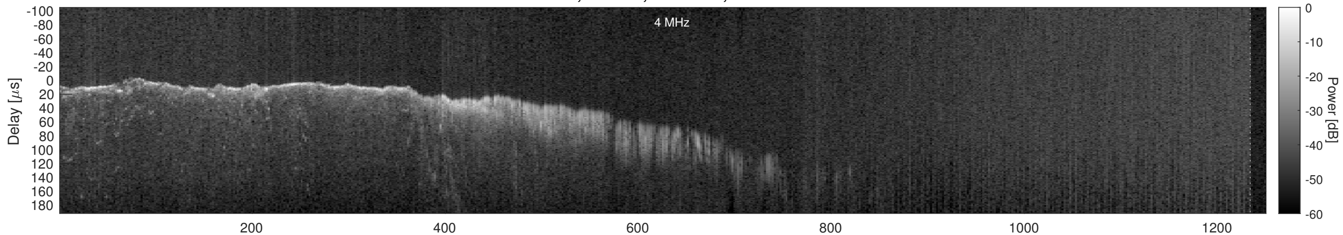
Orbit 2498, Window, Channel 2, Chapman
