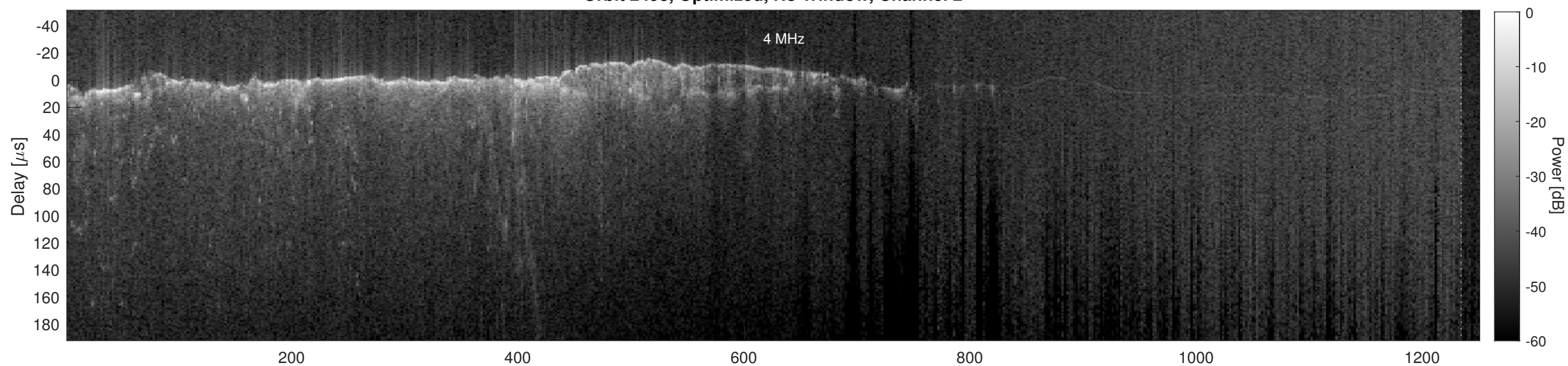
Orbit 2498, Cluttergram
