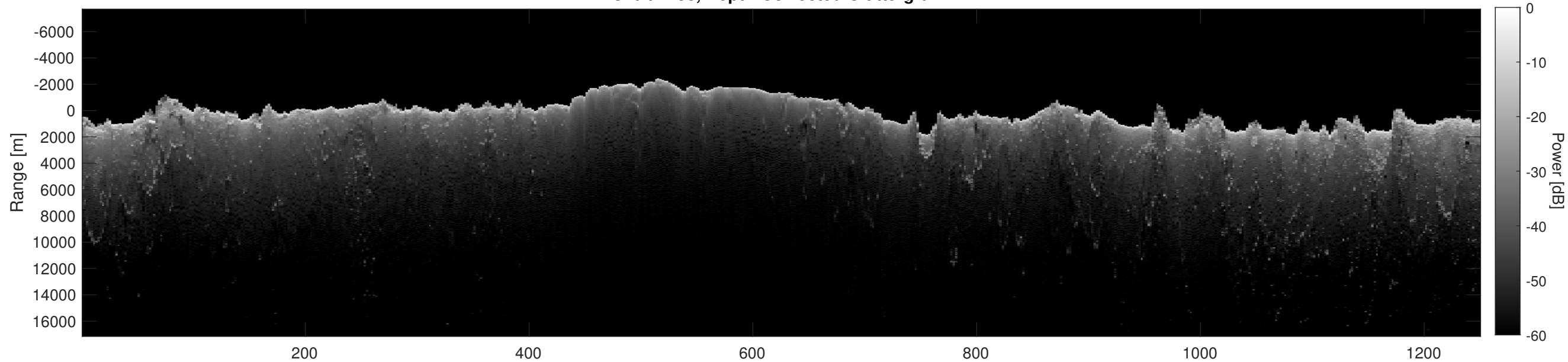
Orbit 2498, Depth-Corrected Cluttergram
