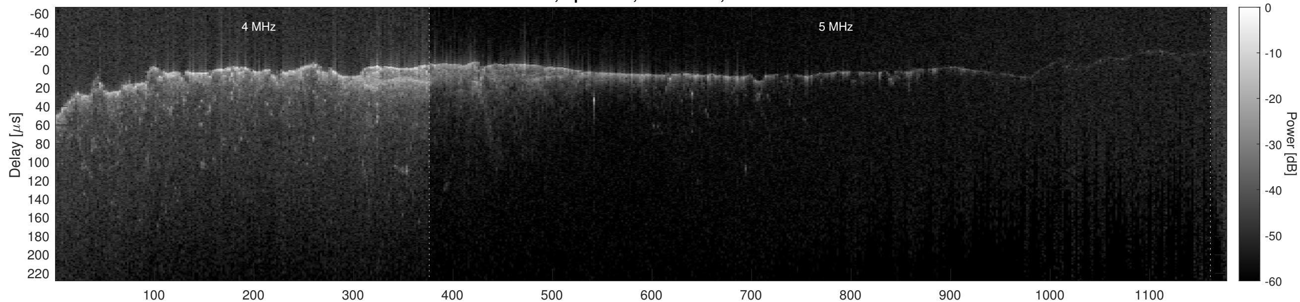
Orbit 2501, Optimized, No Window, Channel 2
