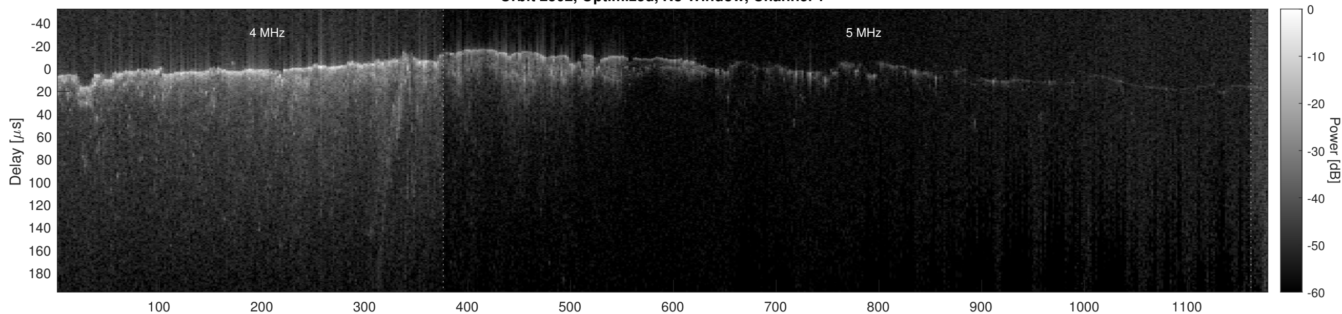
Orbit 2502, Optimized, No Window, Channel 2
