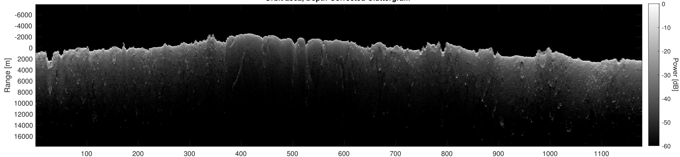
Orbit 2502, Depth-Corrected Cluttergram
