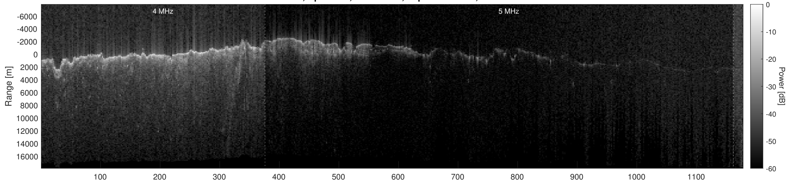
Orbit 2502, Optimized, No Window, Depth-Corrected, Channel 2
