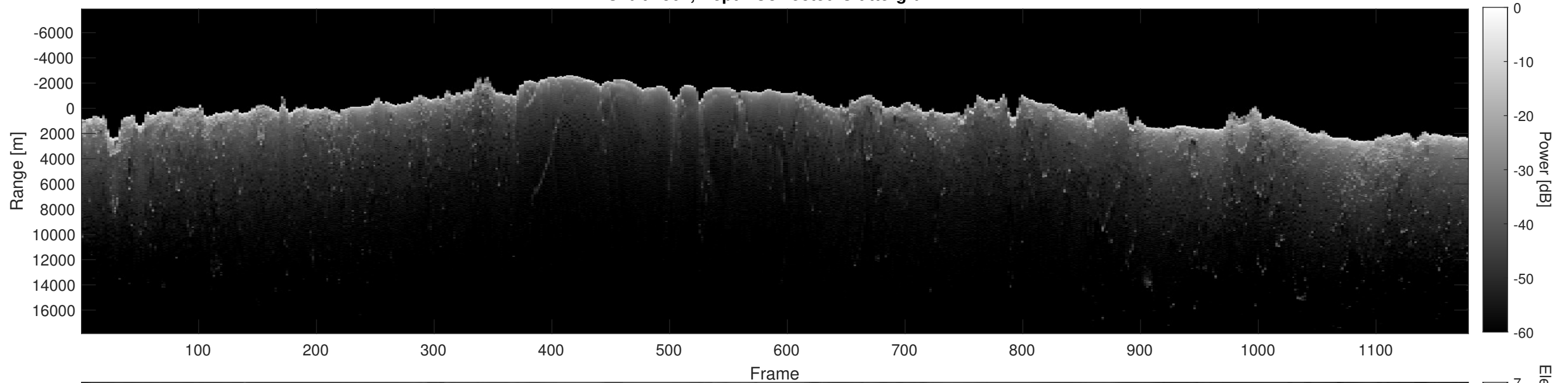
Orbit 2502, Depth-Corrected Cluttergram
