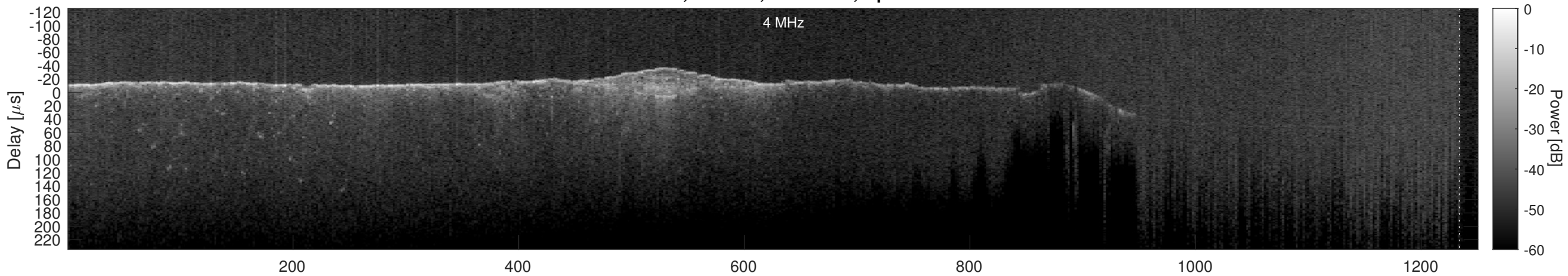
Orbit 2503, Cluttergram
