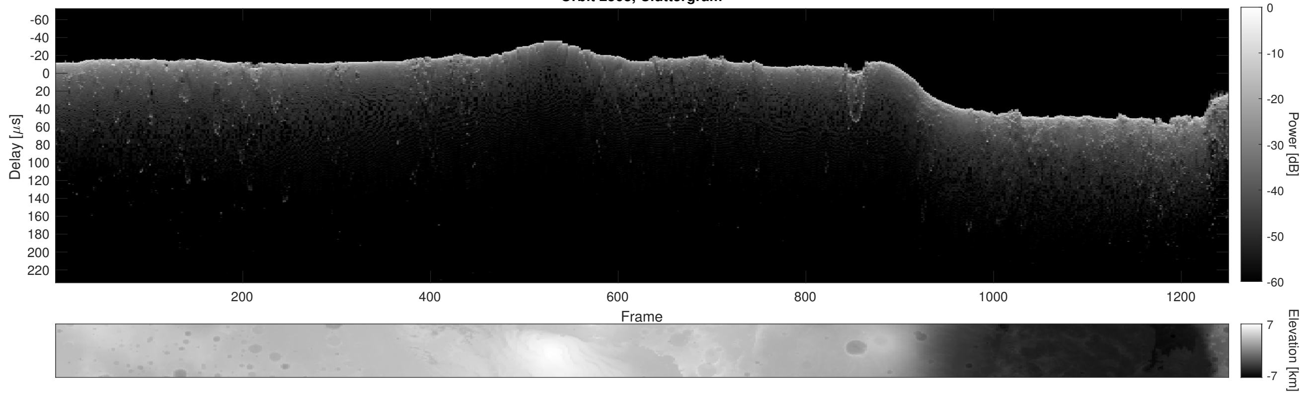
Orbit 2503, Cluttergram
