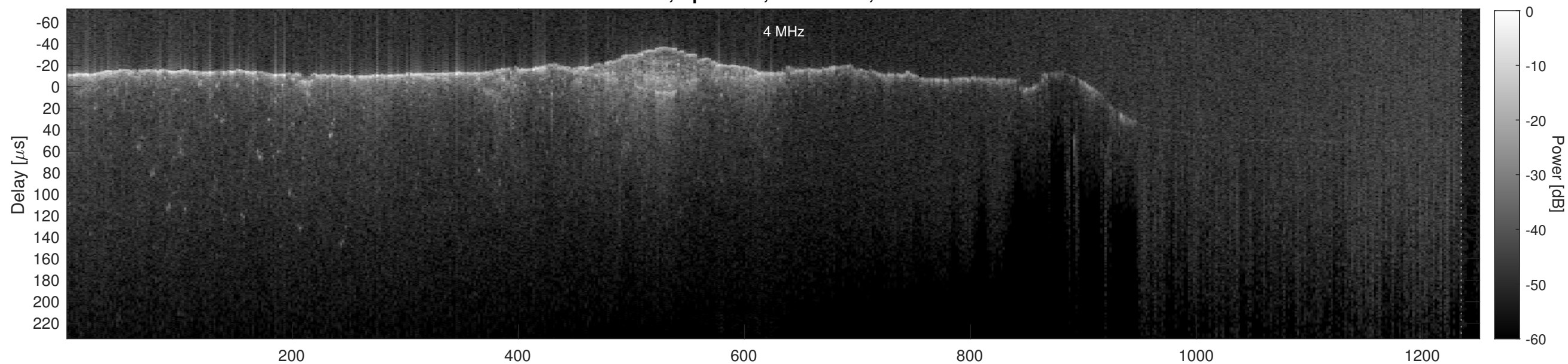
Orbit 2503, Cluttergram
