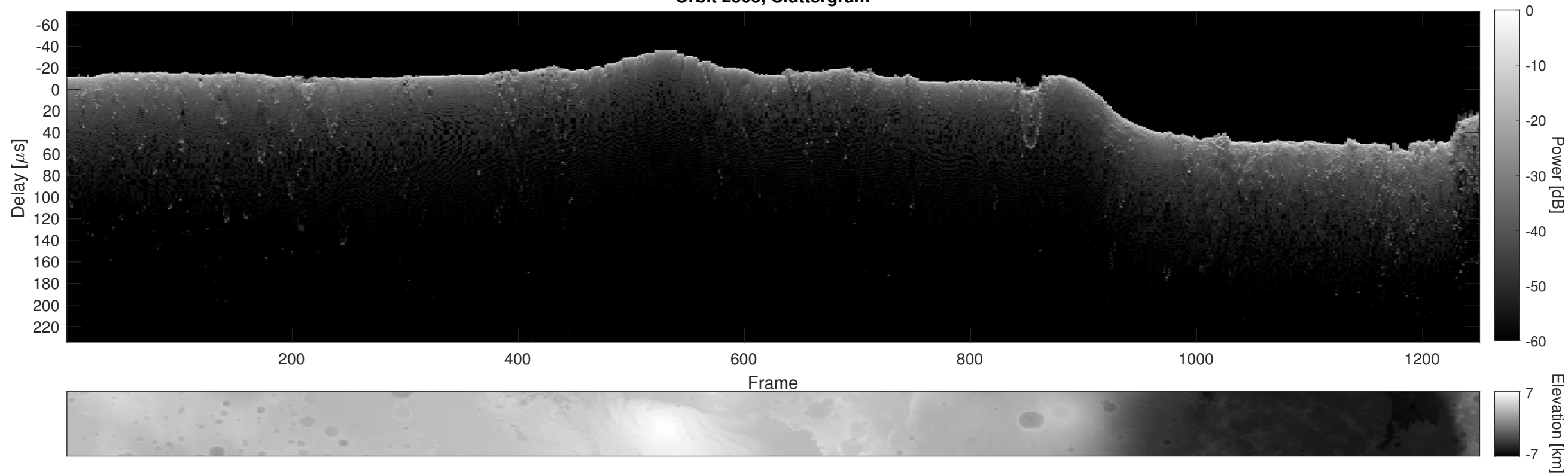
Orbit 2503, Cluttergram
