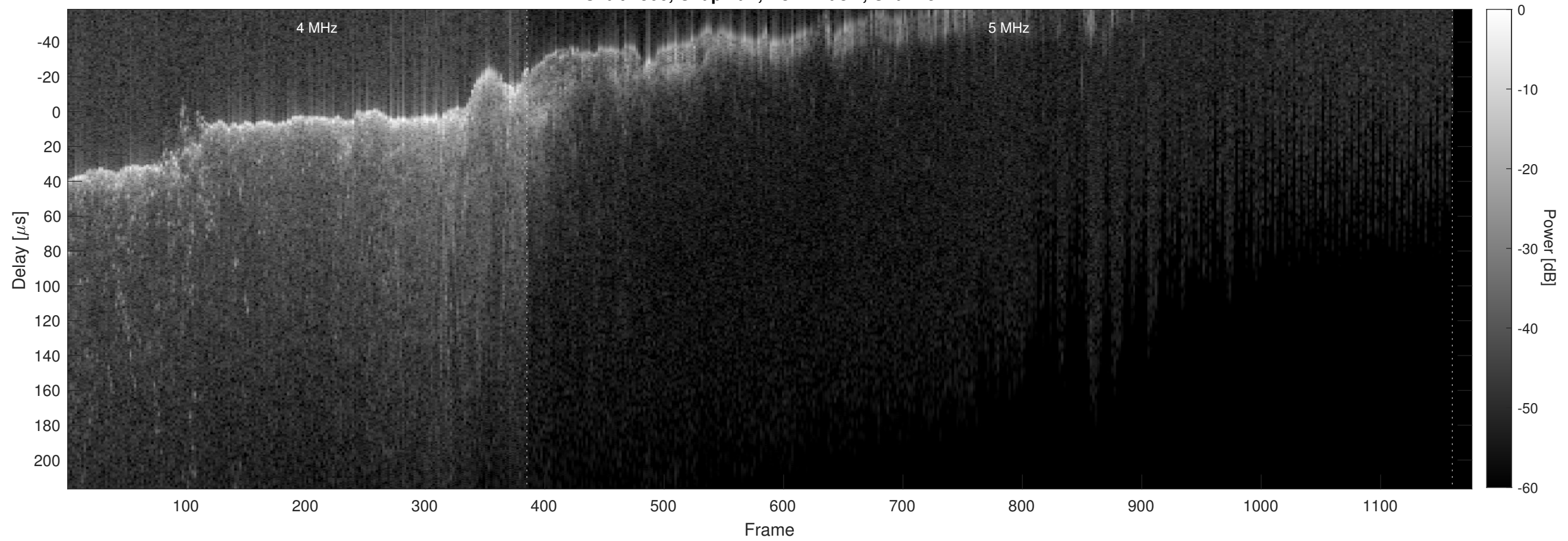
Orbit 2506, Chapman, No Window, Channel 2
