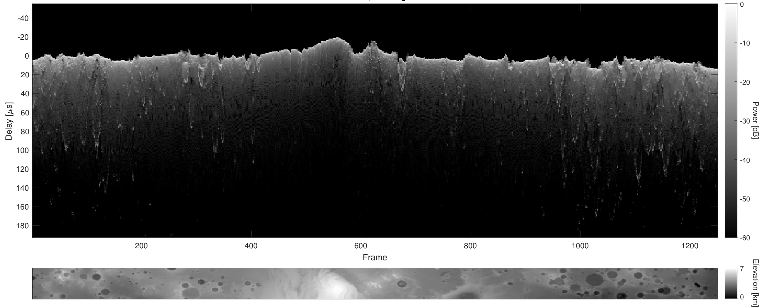
Orbit 2507, Cluttergram
