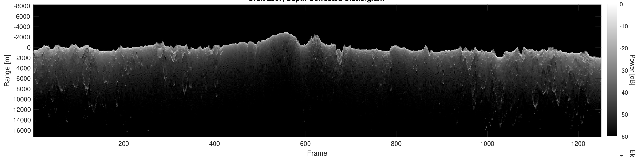
Orbit 2507, Depth-Corrected Cluttergram
