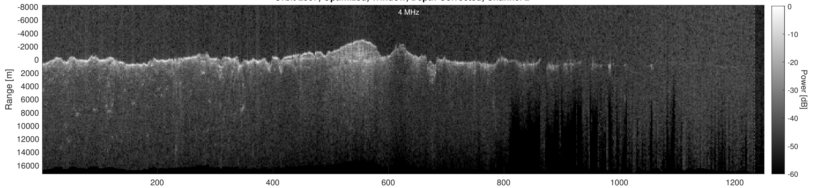
Orbit 2507, Depth-Corrected Cluttergram
