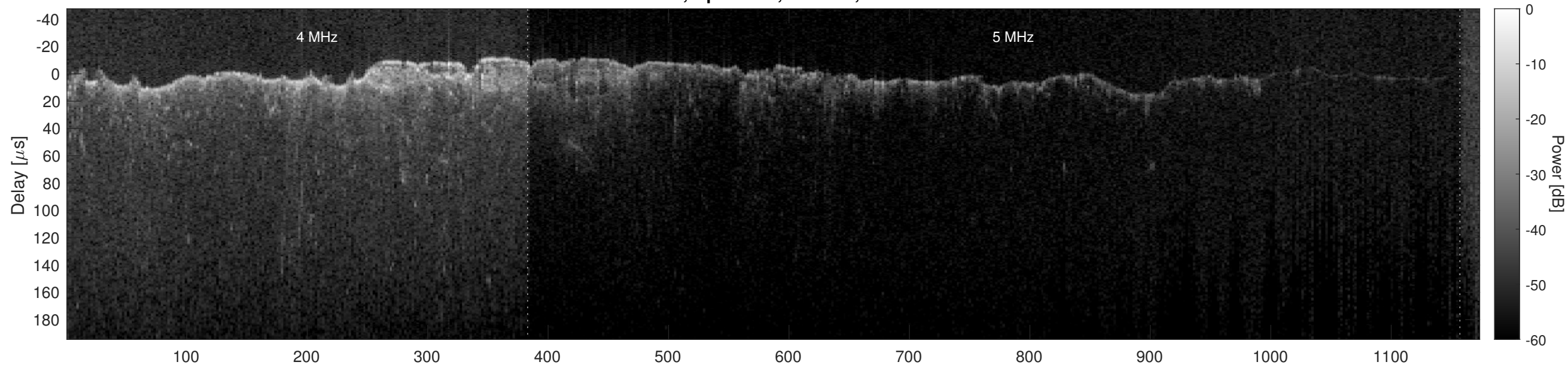
Orbit 2508, Optimized, Window, Channel 2
