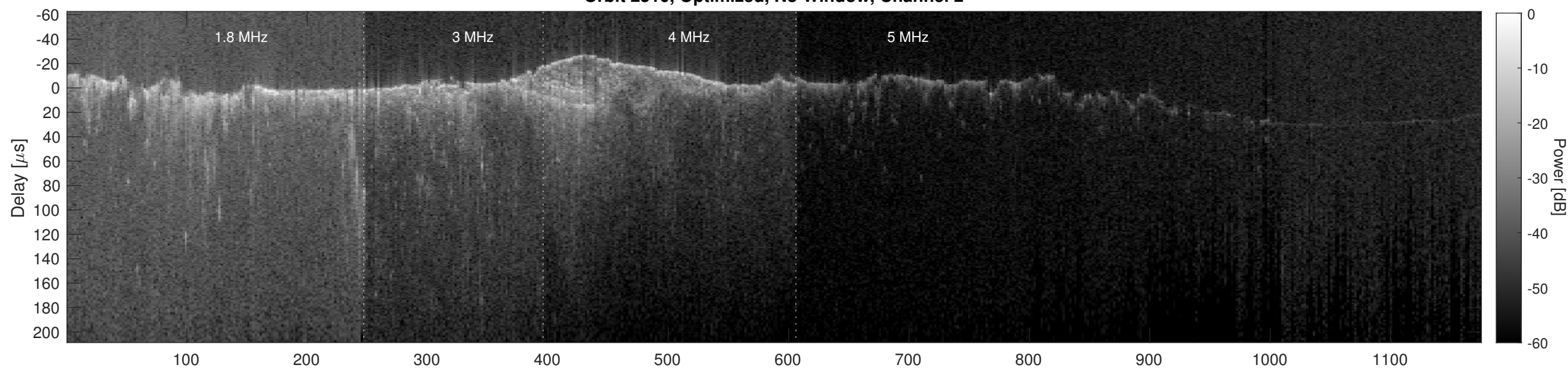
Orbit 2510, Cluttergram
