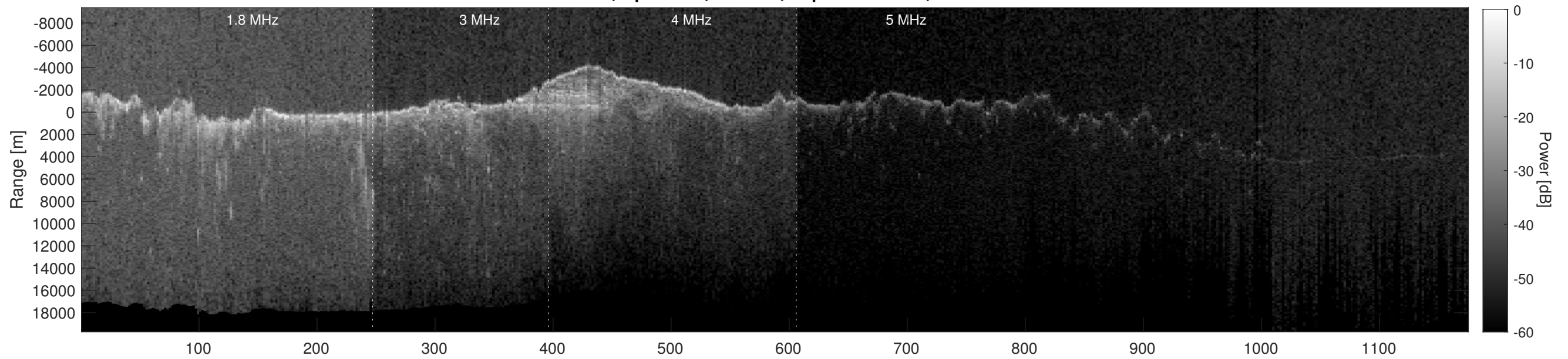
Orbit 2510, Depth-Corrected Cluttergram
