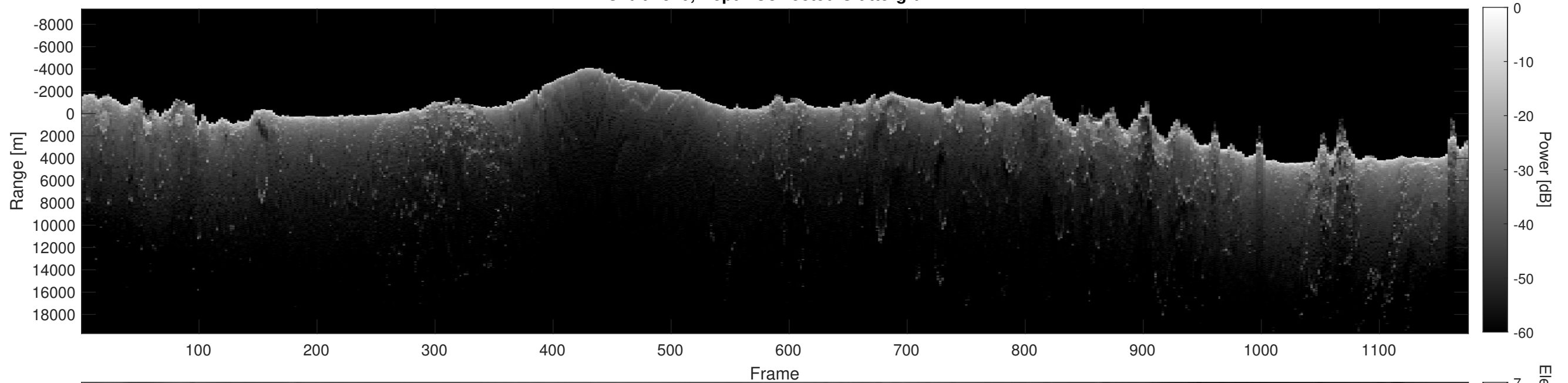
Orbit 2510, Depth-Corrected Cluttergram
