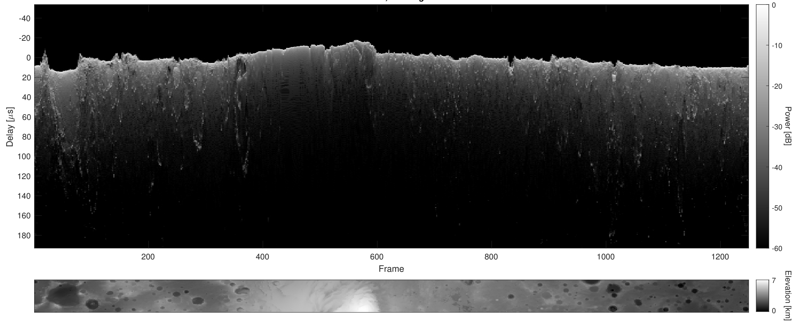
Orbit 2511, Cluttergram
