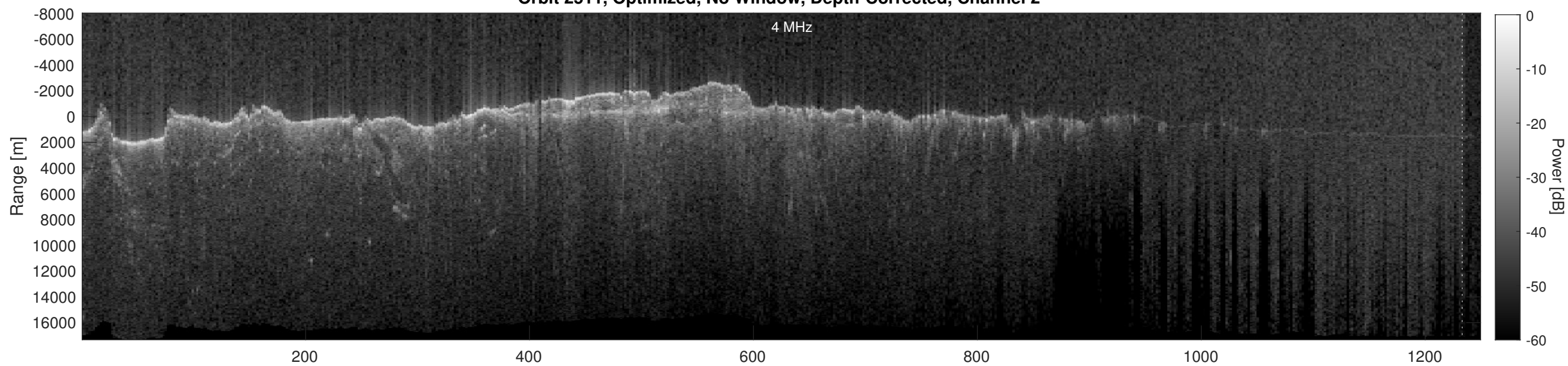
Orbit 2511, Depth-Corrected Cluttergram
