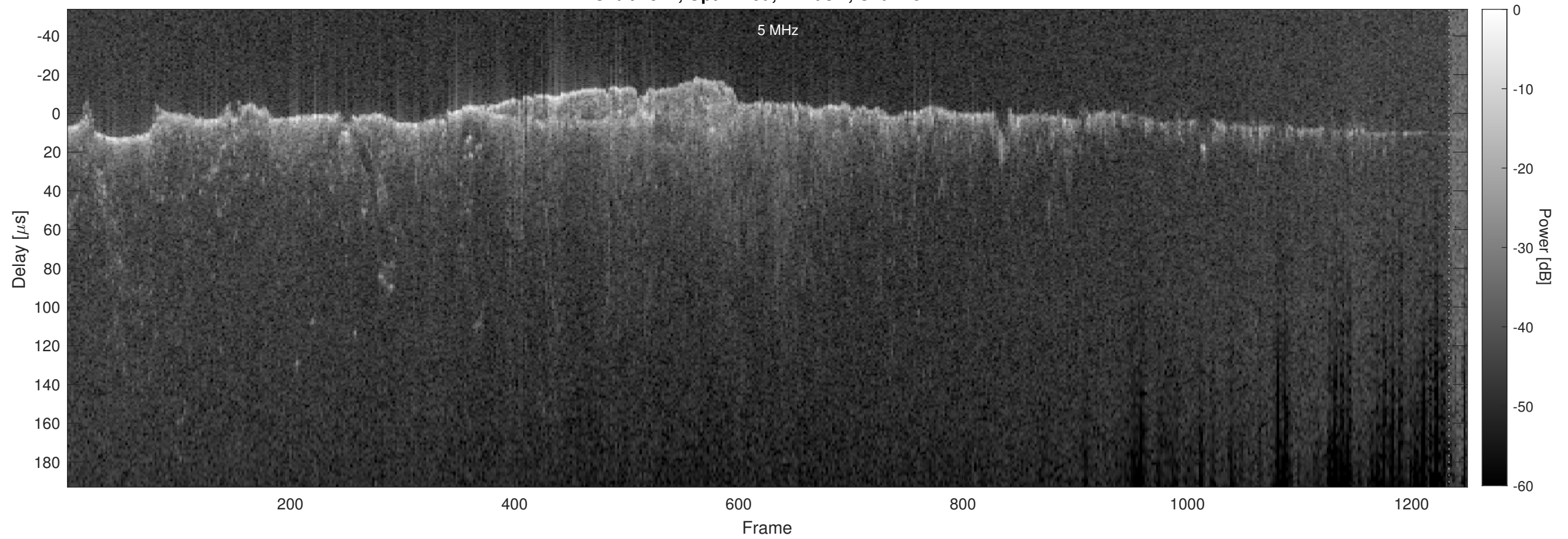
Orbit 2511, Optimized, Window, Channel 2
