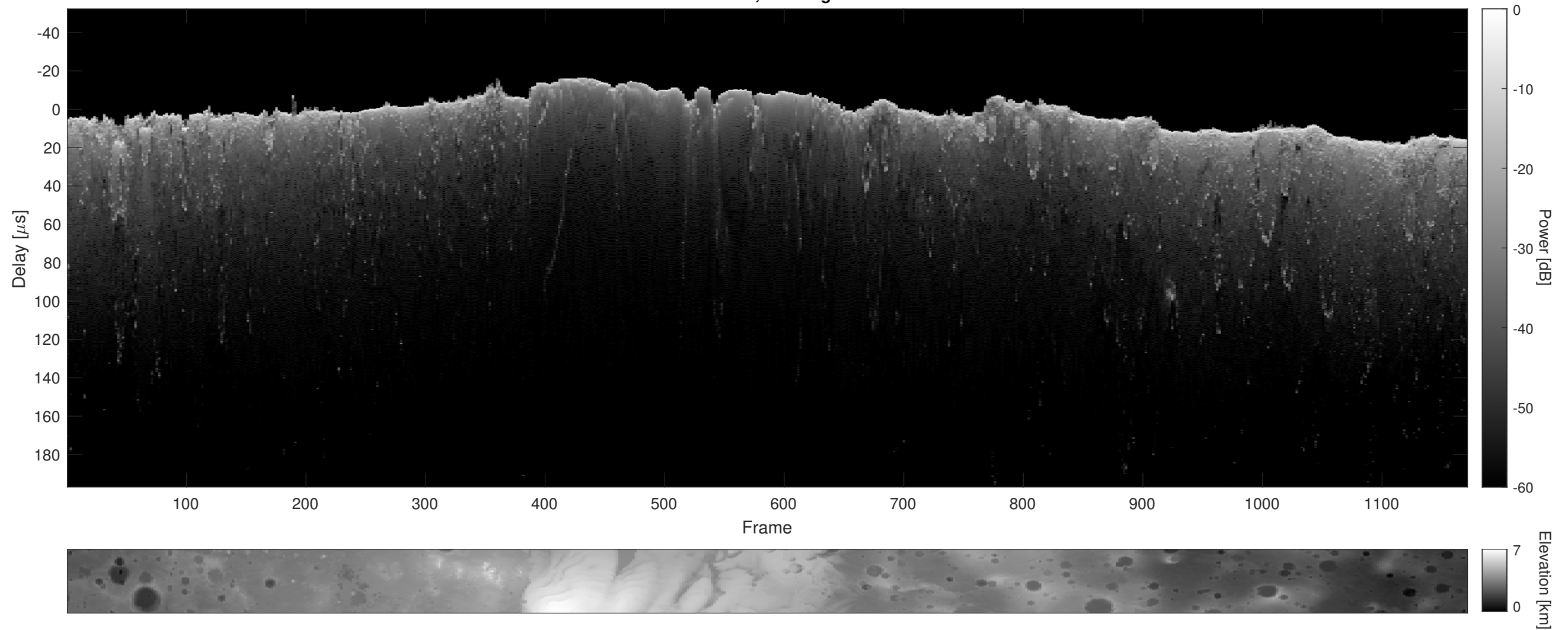
Orbit 2513, Cluttergram
