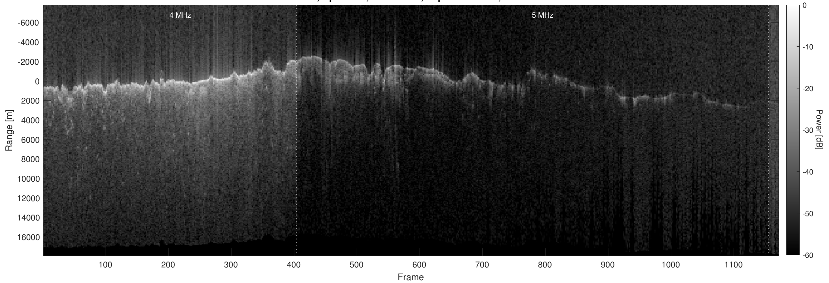
Orbit 2513, Optimized, No Window, Depth-Corrected, Channel 2
