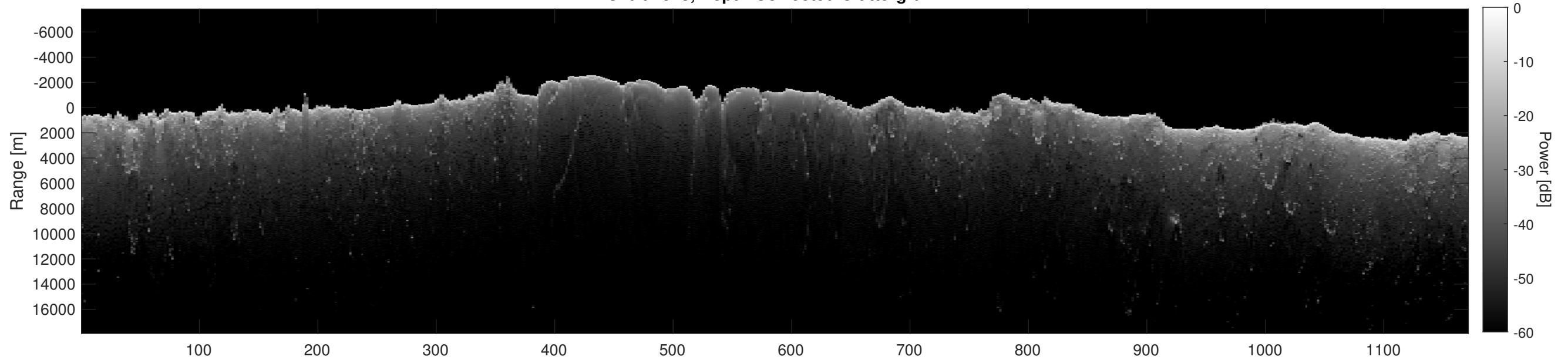
Orbit 2513, Depth-Corrected Cluttergram
