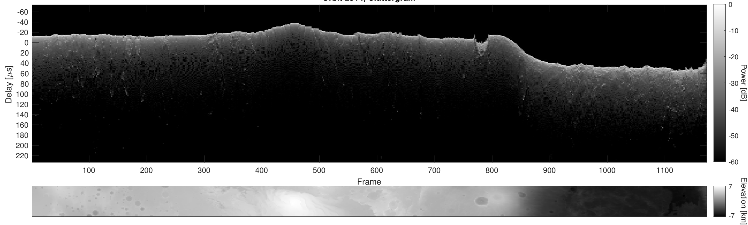
Orbit 2514, Cluttergram
