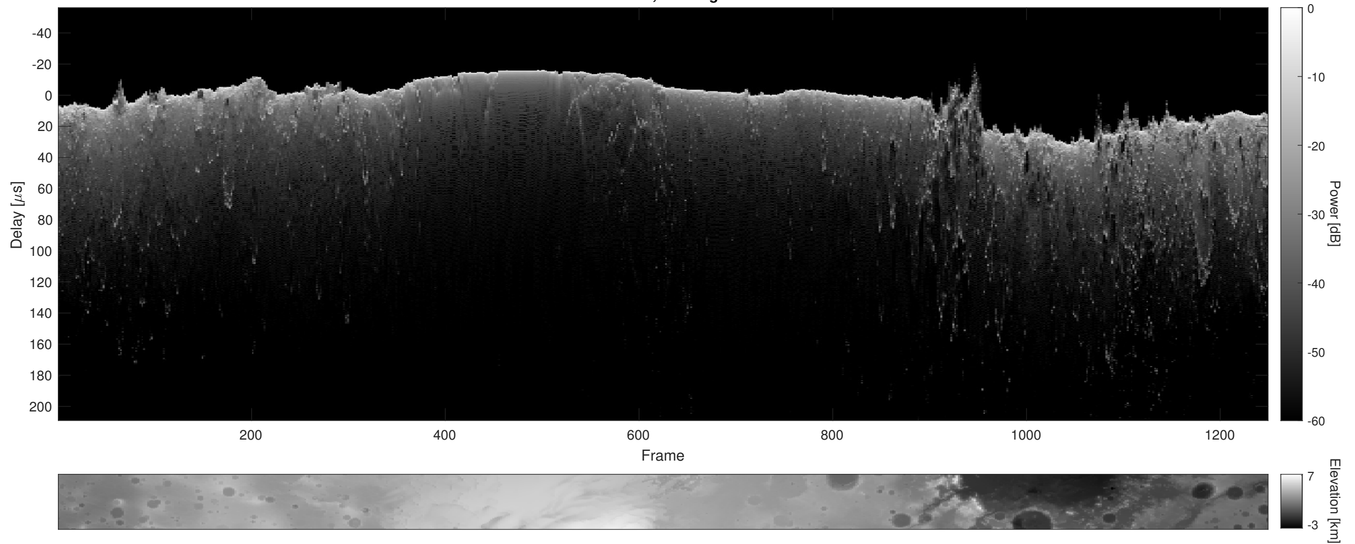
Orbit 2515, Cluttergram
