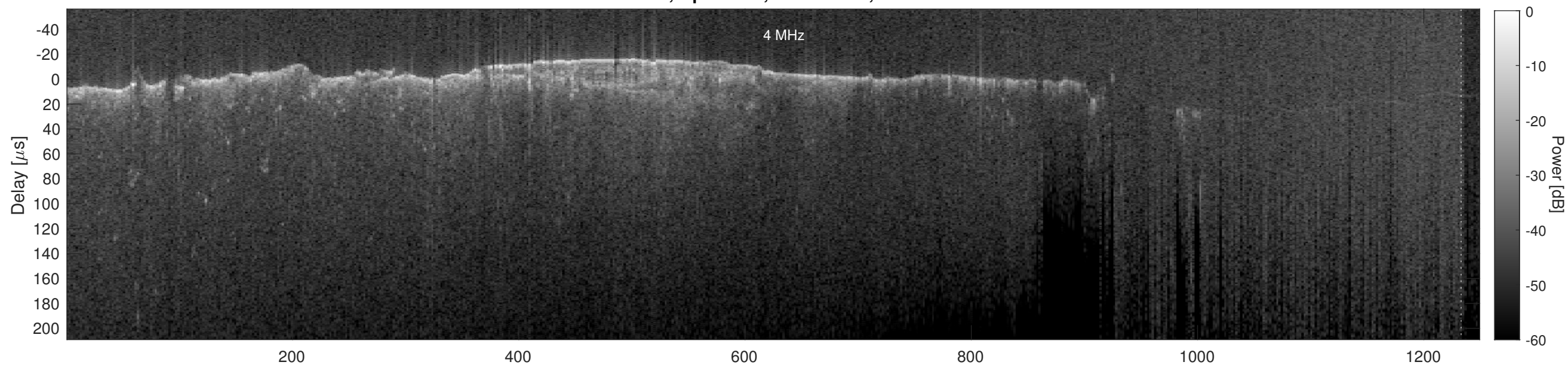
Orbit 2515, Cluttergram
